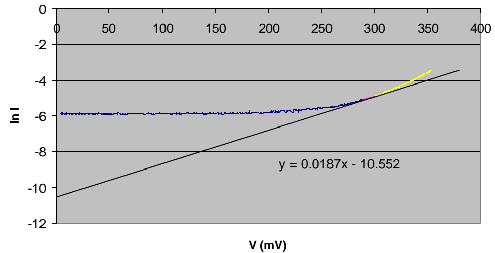
In I vs V (rendah)
